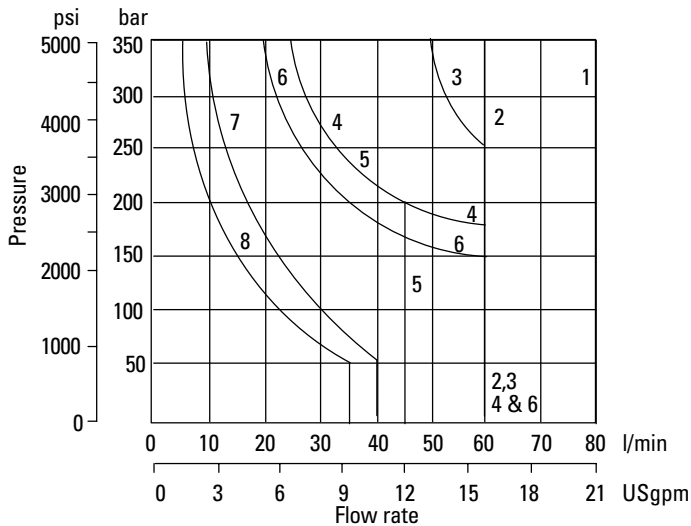
Graph 6 DC solenoid valves
