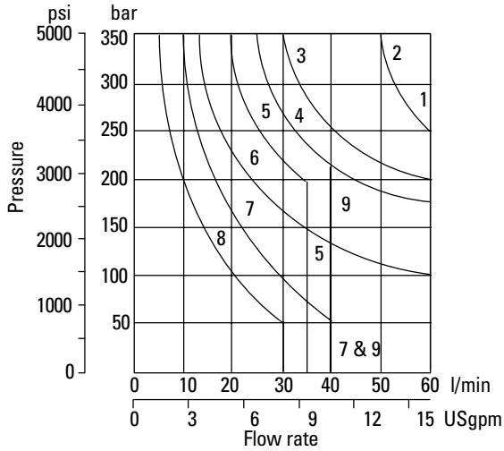
Graph 4 – Single-frequency coils AC solenoid valves with: – Dual-frequency coils operating at 50 Hz
