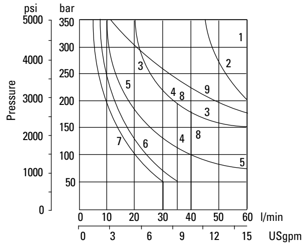
Graph 5 AC solenoid valves with dual-frequency coils operating at 60 Hz
