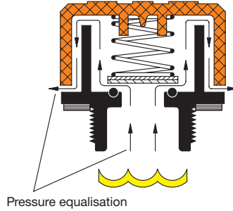
ELESA Original design SFV.
